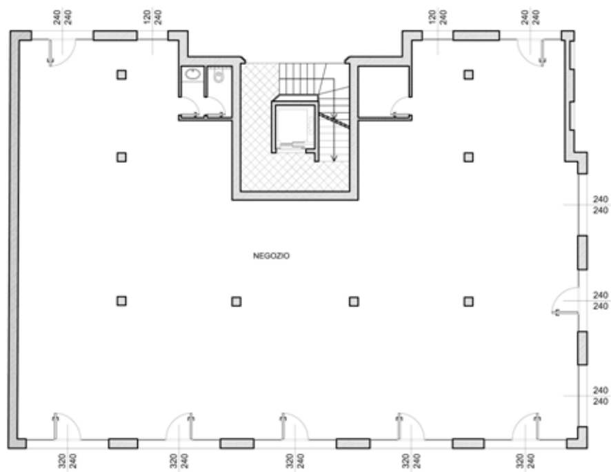
Piano Terra
