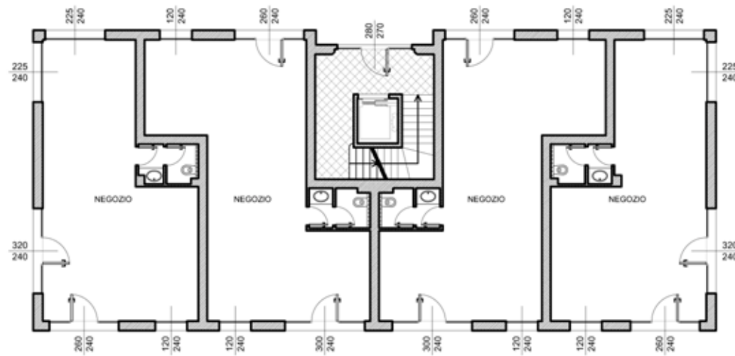
Piano Terra
